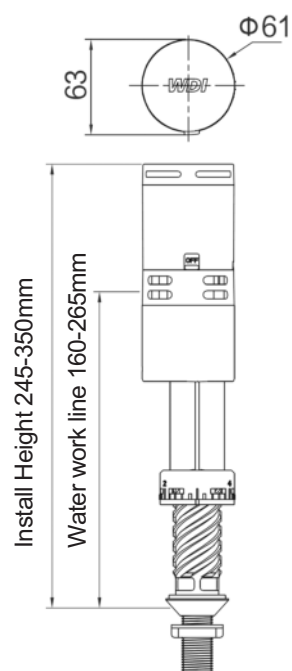
Brass tail with rapid fix installation that includes slideable locking nut
